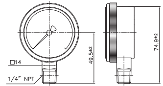
NPT MALE
