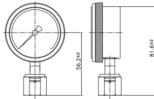
SWIVEL FEMALE
