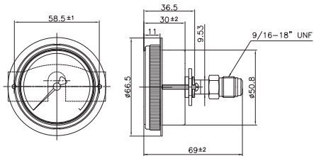
SWIVEL MALE
