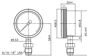
SWIVEL MALE
